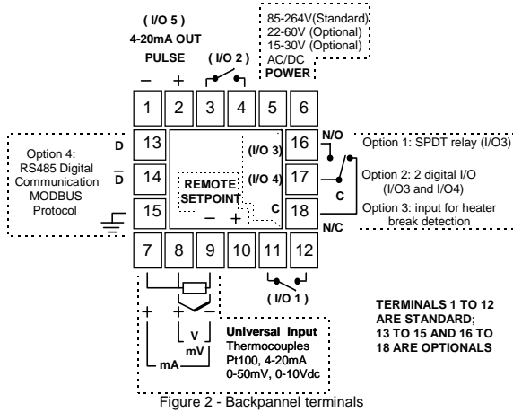
Figure 2 - Backpanel terminals
