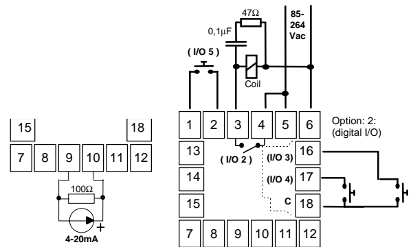
Figure 7 - remote SP input
