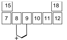
Figure 3 - thermocouple wiring
