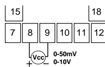
Figure 4 - voltage input wiring
