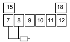
Figure 5 - 3 wire Pt100
